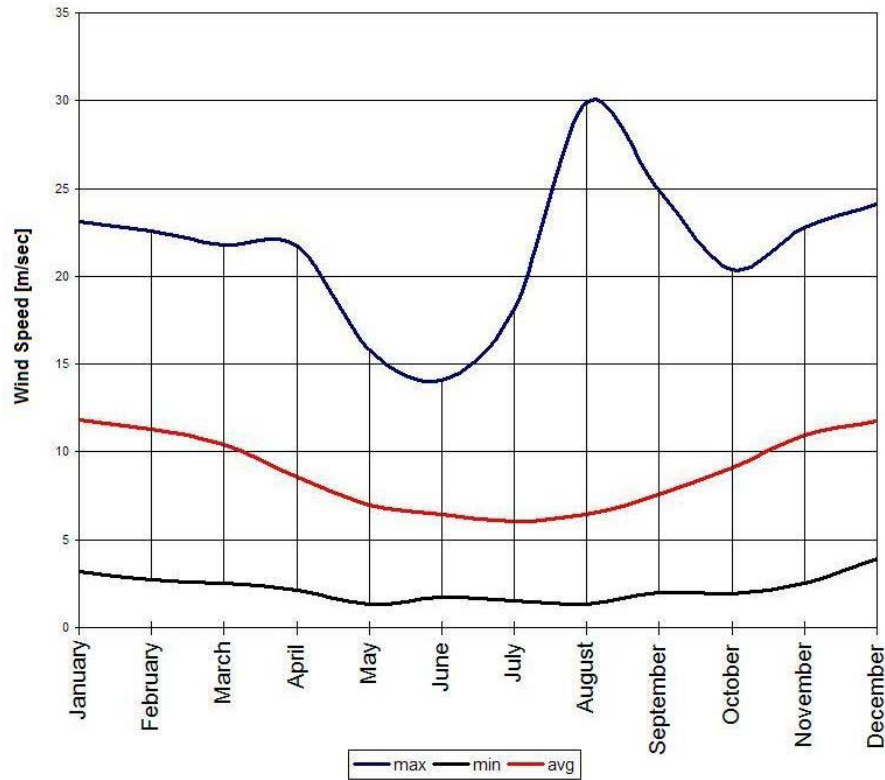
Figure 2.5. Average annual, average maximum, and average minimum wind speeds over the Ocean SAMP area. (Spaulding 2007).
