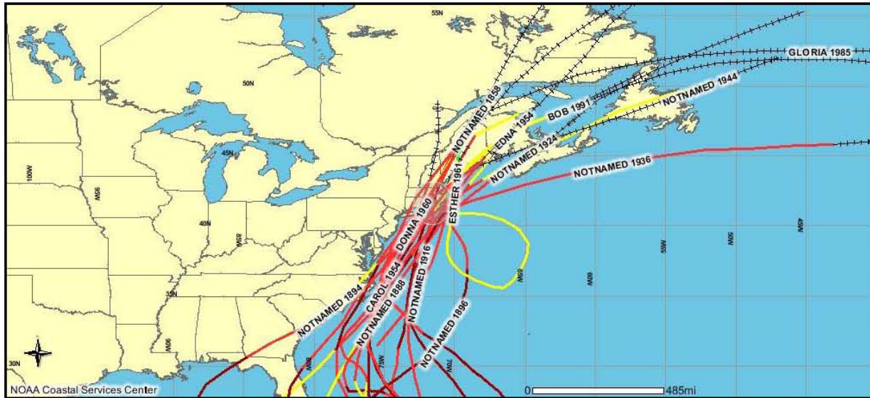
Figure 2.6. Hurricane tracks where the eye moved over Rhode Island, intersecting the Ocean SAMP area (NOAA Coastal Services Center n.d.).
