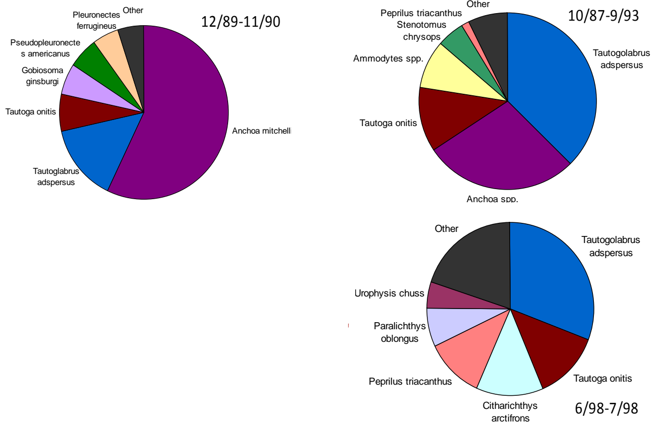
Figure 2.23. Ichthyoplankton abundance at the mouth of Narragansett Bay/Rhode Island Sound at various points in time (from Pfeiffer-Herbert 2009).
