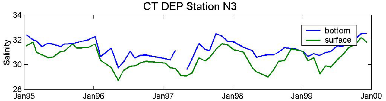
Figure 2.13. Average annual surface and bottom salinity at a station in Block Island Sound (CTDEP No. N3; between NW of BI, 3/4 of the way to The Race; from O’Donnell and Houk 2009). Periods where surface and bottom salinities are nearly equal suggest mixing events, while rapid declines in salinity of surface waters suggests increased freshwater input associated with increased runoff in rivers feeding Long Island Sound.
