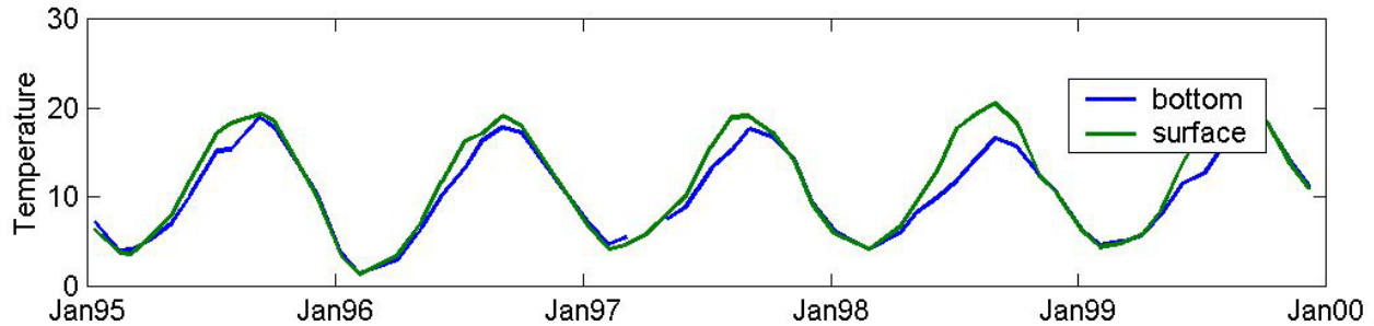
Figure 2.11. Average annual surface and bottom temperatures at a station in Block Island Sound (CTDEP No. N3; between NW of BI, ¾ of the way to The Race; from O’Donnell and Houk 2009).
