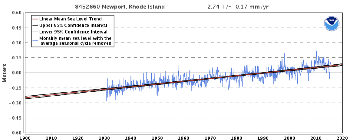
Figure 1. Sea level has risen 9.1 inches since 1930 based on the long-term trend at Newport.
