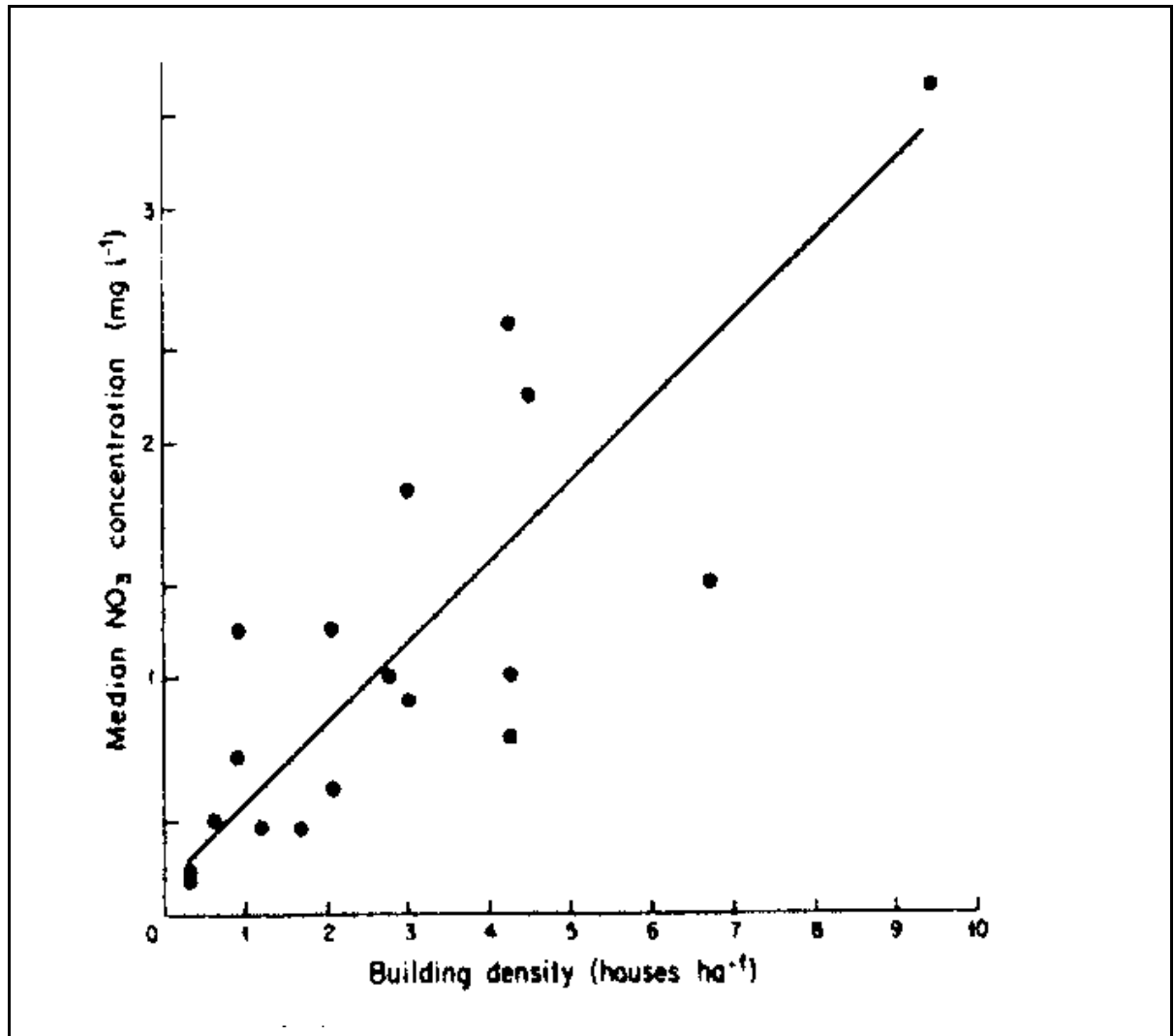
Figure 3-8. Median nitrate ( \text{NO}_3 ) concentrations in groundwater beneath areas of Cape Cod with different building densities (Persky 1986).
