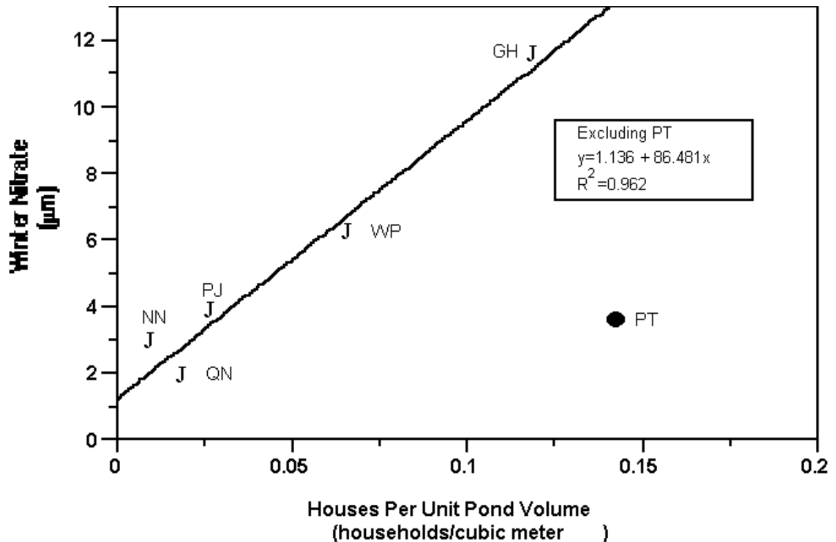
Figure 3-13. Winter nitrate (Fm) levels compared to housing per unit pond volume (houses/m 3 ).
