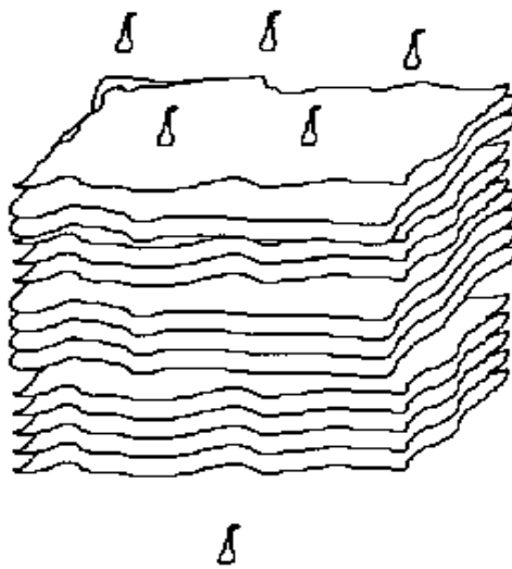
Platy Structure
