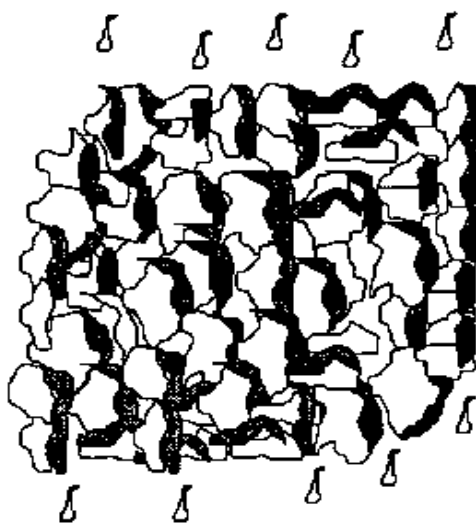
Blocky Structure
