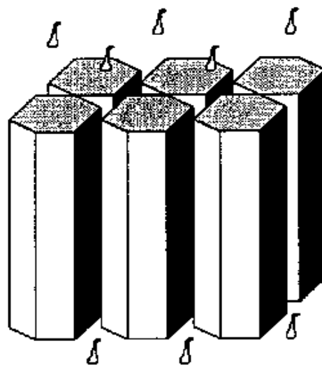
Prismatic Structure
